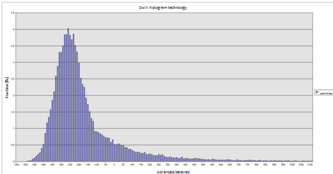
Figure 7: Typical turbulence measured at an paintshop area
